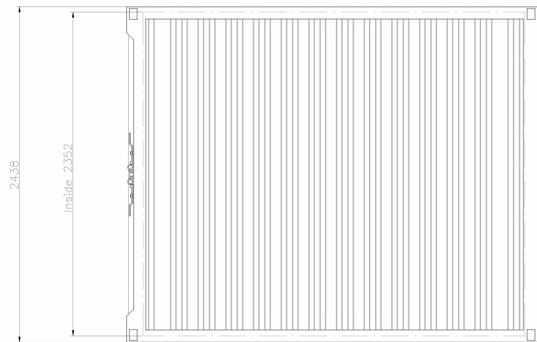
Top view
