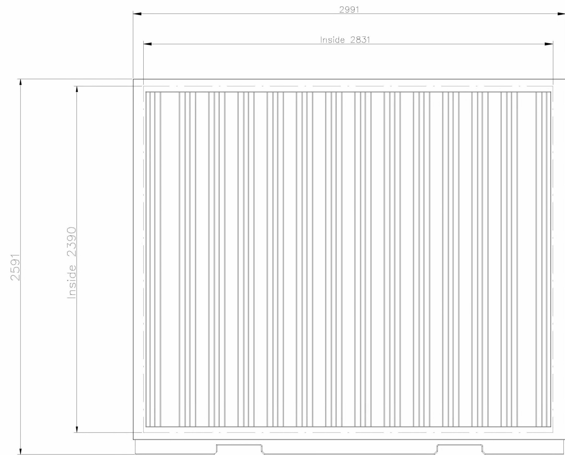
side view
