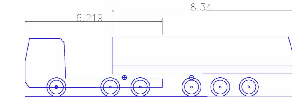
mover Overall Length 12.289m
