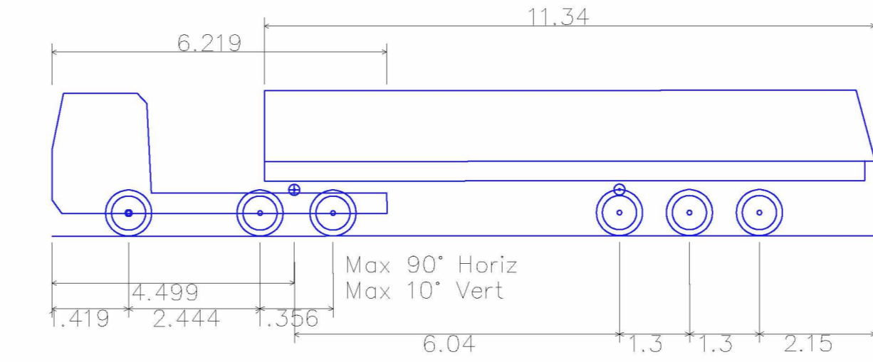
Tanker (Conform ASVV) Overall Length 15.289m
